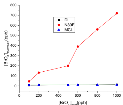
Fig.3 : Effect of variation of bromate concentration on the bromate rejection by the nanofiltration membranes (T=25°C ;P=6 bar,pH=8).
