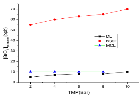
Fig.2 : [BrO 3 - ] permeate versus hydraulic pressure ([BrO 3 - ] feed =100 ppb,pH=8).
