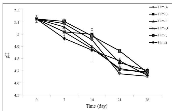
Figure 1. Changes in the pH values of the Iranian Traditional cheese packaged in nanocomposite films during 28 days storage period at 5°C
