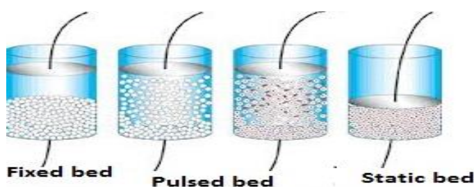
Figure 1: Schematic diagram of hydraulic motion of resin in different beds
