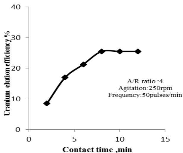
5. Figure 9: Effect of contact time on Uranium elution efficiency
