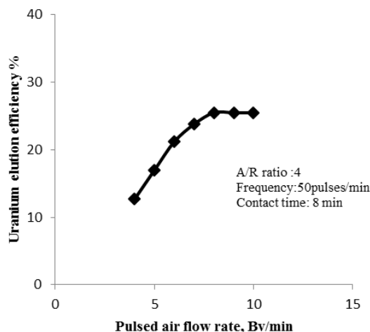
Figure 10: Effect of pulsed air flow rate on uranium elution efficiency
