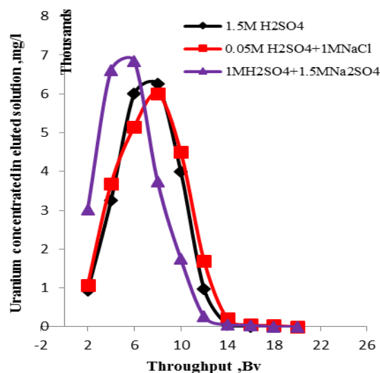
Figure 13: Uranium elution peak concentrations
