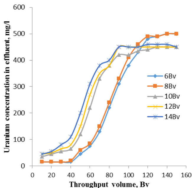
Figure 6: Breakthrough profiles for different flow rates
