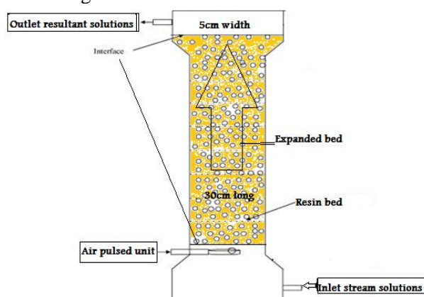
Figure2: Schematic flow diagram of air pulsed Column
