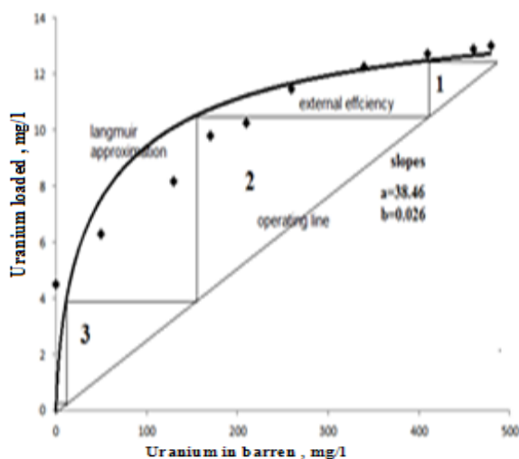
Figure 7: Uranium adsorption isotherm
