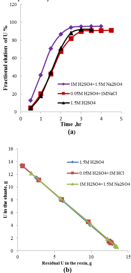
Figure 14: Equilibrium isotherm and kinetics of uranium elution by different eluent in air pulsed column
