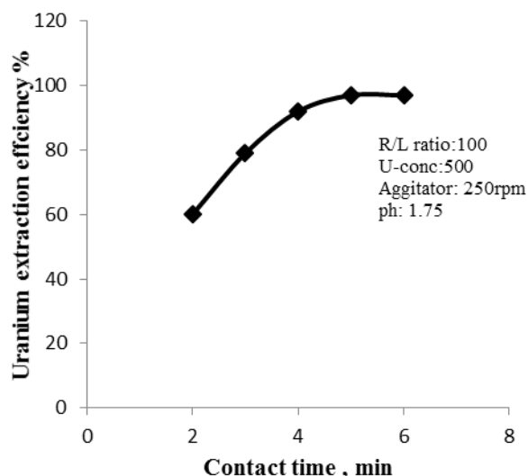
Figure 3: Effect of contact time on uranium extraction efficiency%
