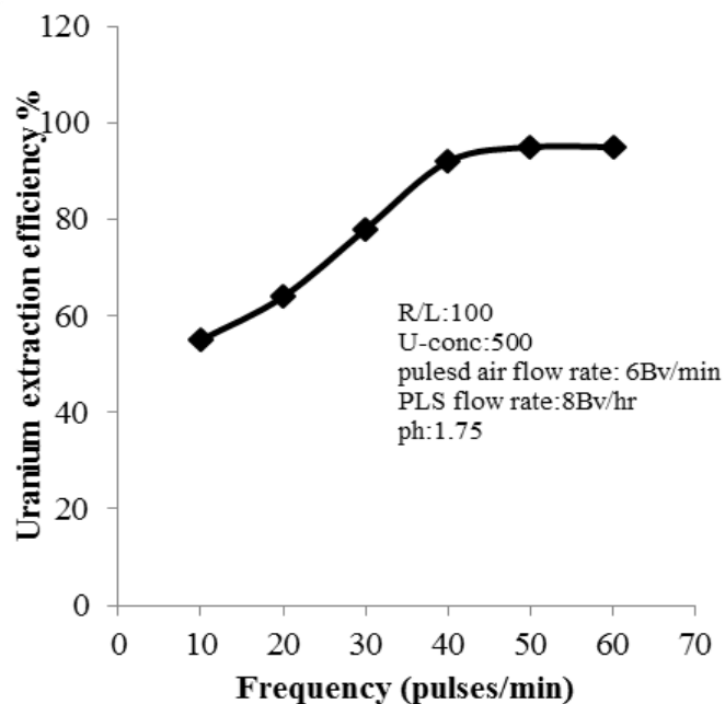
Figure 5: Effect of frequency on uranium extraction efficiency%
