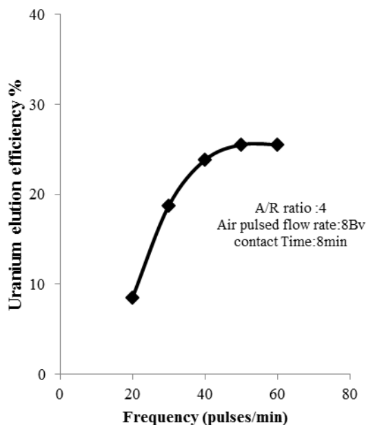
Figure 11: Effect of pulsed air frequency on Uranium elution efficiency
