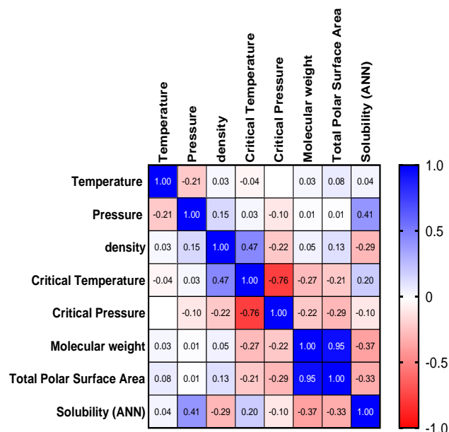
Figure-3: Heat map chart of the Pearson product moment correlation analysis performed on the input and output variables of the FFBP-ANN model.
