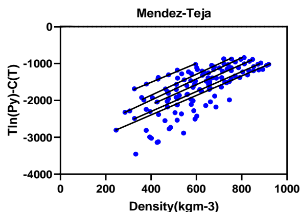
Figure-4: Solubility of the investigated dye sample in supercritical carbon dioxide with ethanol as the cosolvent as a function of carbon dioxide density based on the Mendez-Teja model. The trendlines depict the various dye-specific quantities of the cosolvent used during the experiments.
