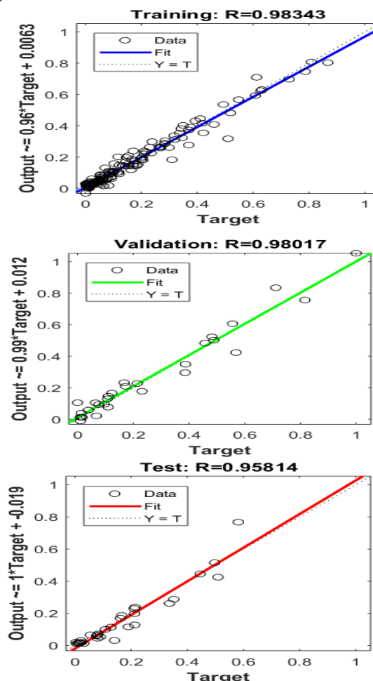
Figure-1: Individual regression plots pertaining to the training, validation and testing of the sample data for the ANN simulation of the (7-7-1) architecture.
