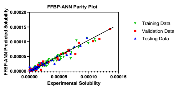
Figure-2: Consolidated experimental v/s FFB-ANN predicted data parity plot of the (7-7-1) architecture ANN simulation.
