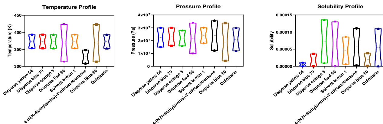
Figure-6 (Enlarged): Parameter profile violin plots illustrating the dye specific ranges of temperature, pressure and solubility.
