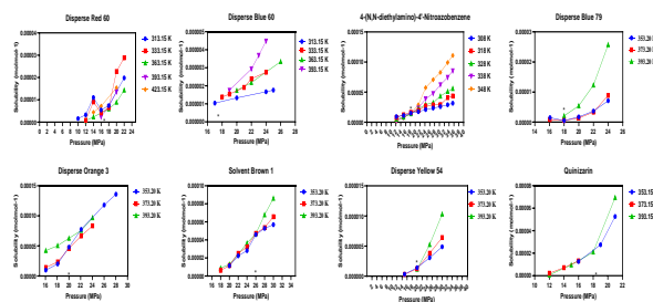
Figure-8: Dye specific isotherm plots that illustrate crossover points (*).
