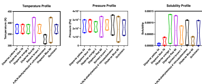
Figure-7: Parameter profile violin plots illustrating the dye specific ranges of temperature, pressure and solubility.
