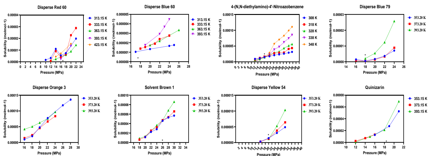
Figure-5 (Enlarged): Dye specific isotherm plots that illustrate crossover points (*).
