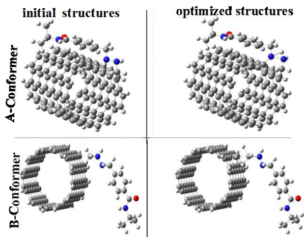
Figure 2. The initial and optimized structures of PC-SWCN complexes
