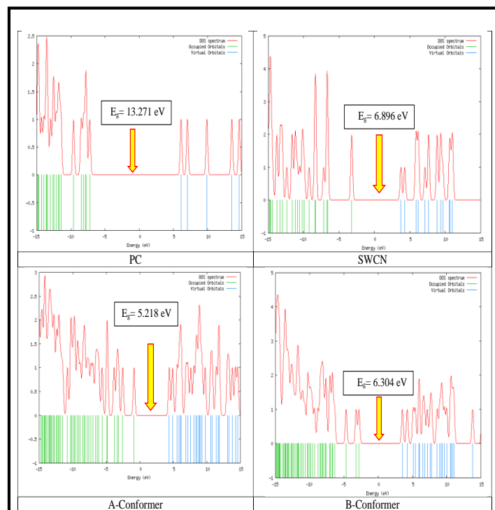
Figure 3. The DOS spectrums of PC, SWCN and their complexes
